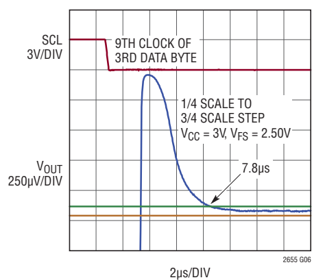
Settling to \pm 1\text{LSB} Rising
