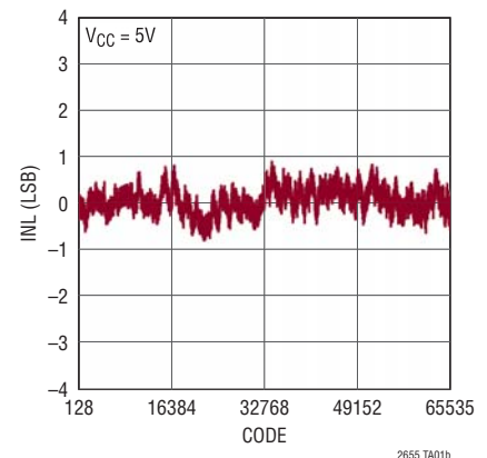
INL Curve
